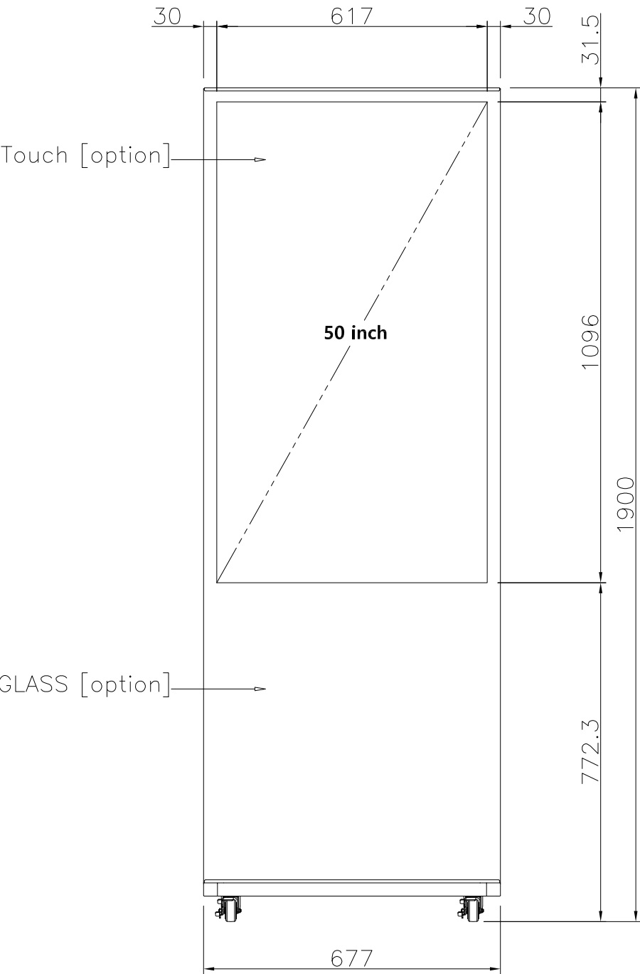
FRONT VIEW
